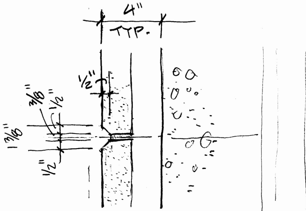
① TYPICAL JOINT
