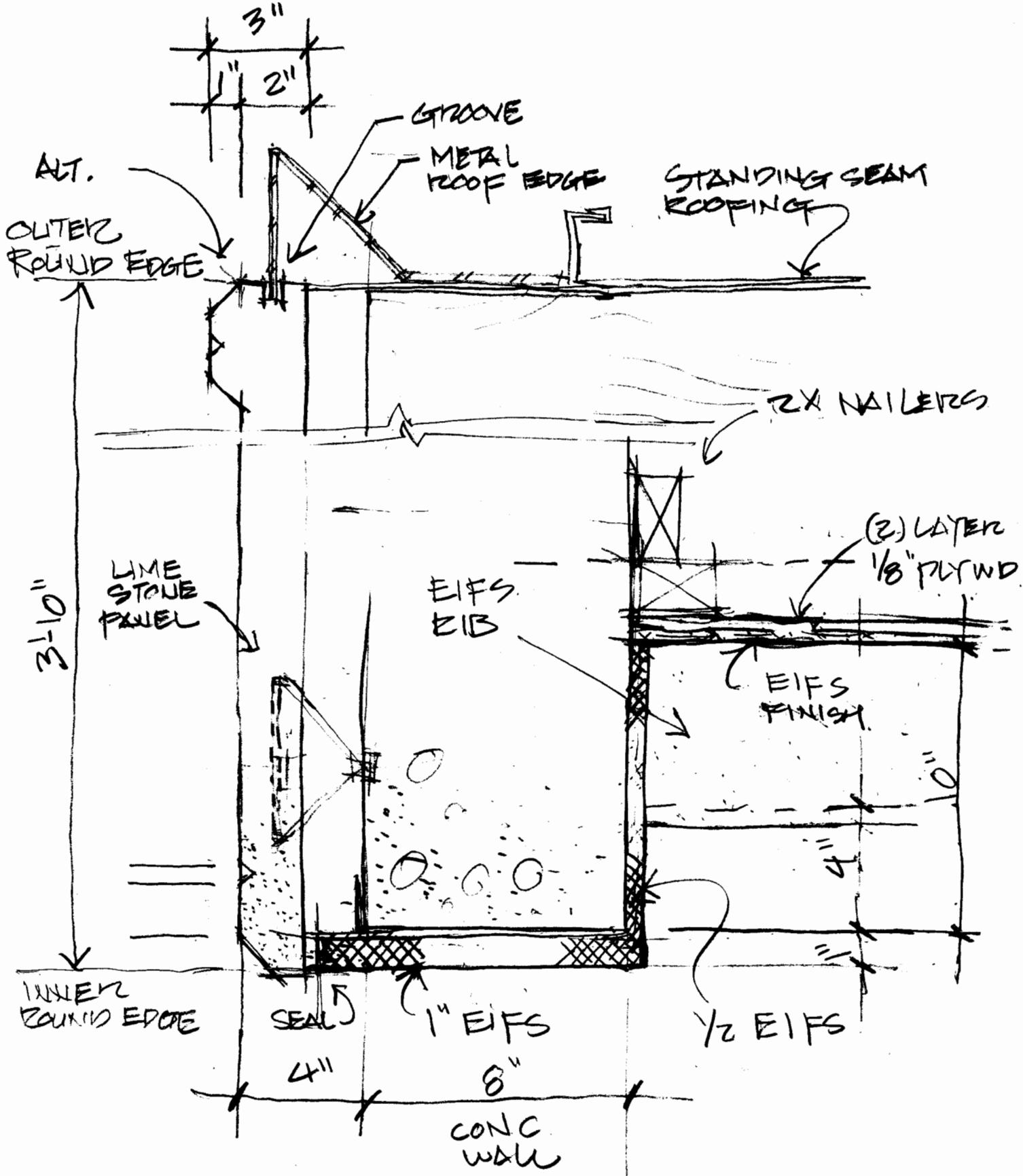
5 CORNER DETAIL
