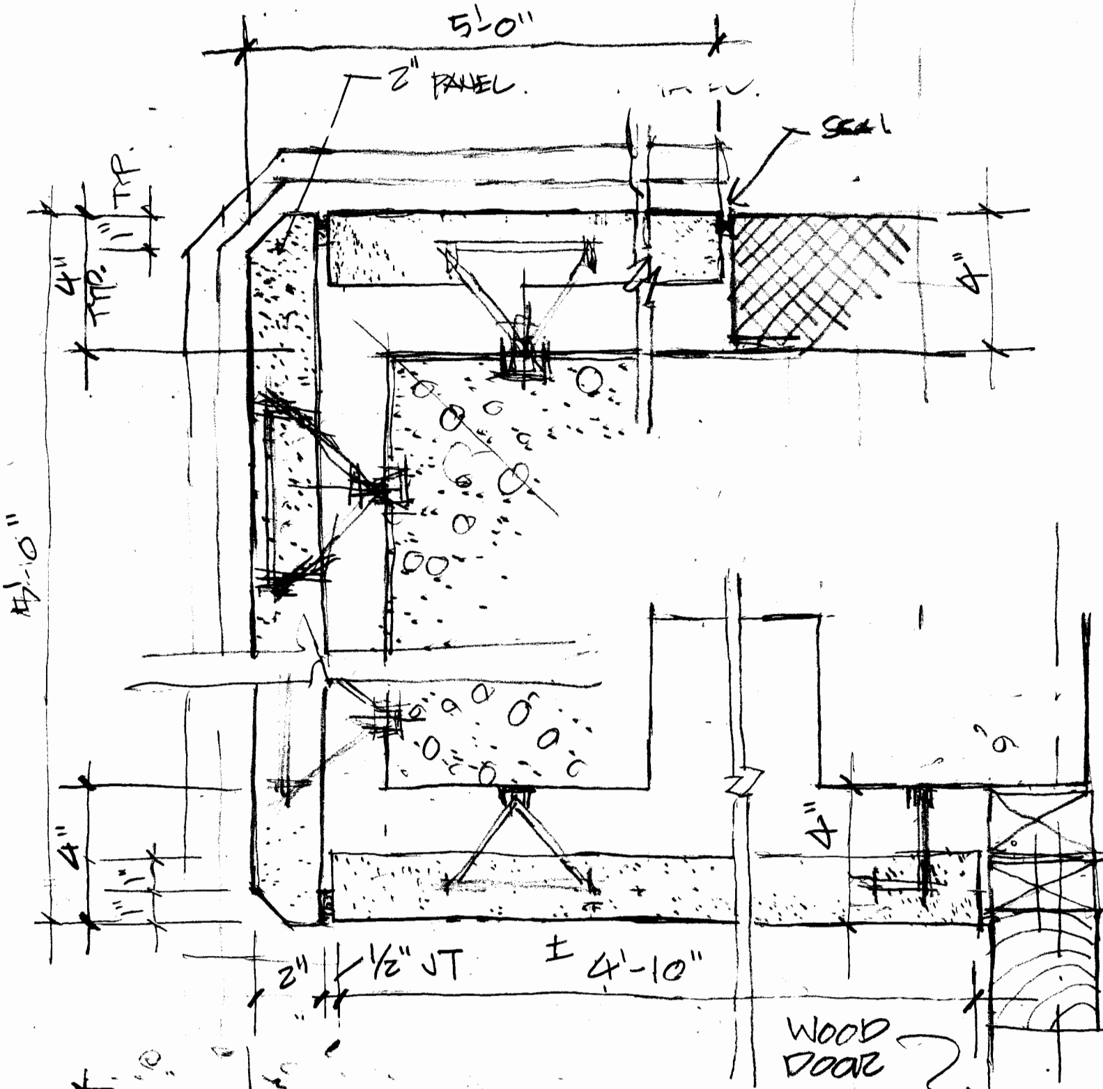
② PLAN DETAIL
