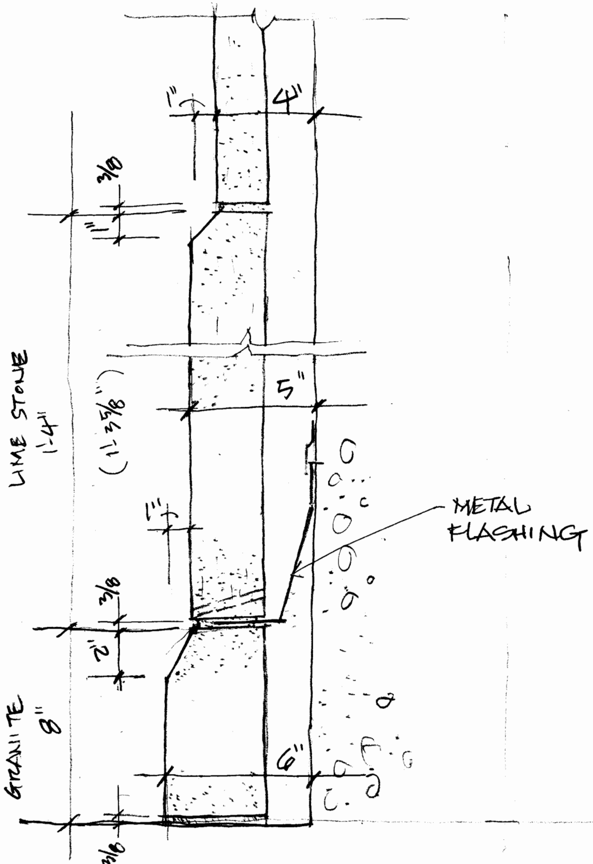
③ BASE DETAIL
