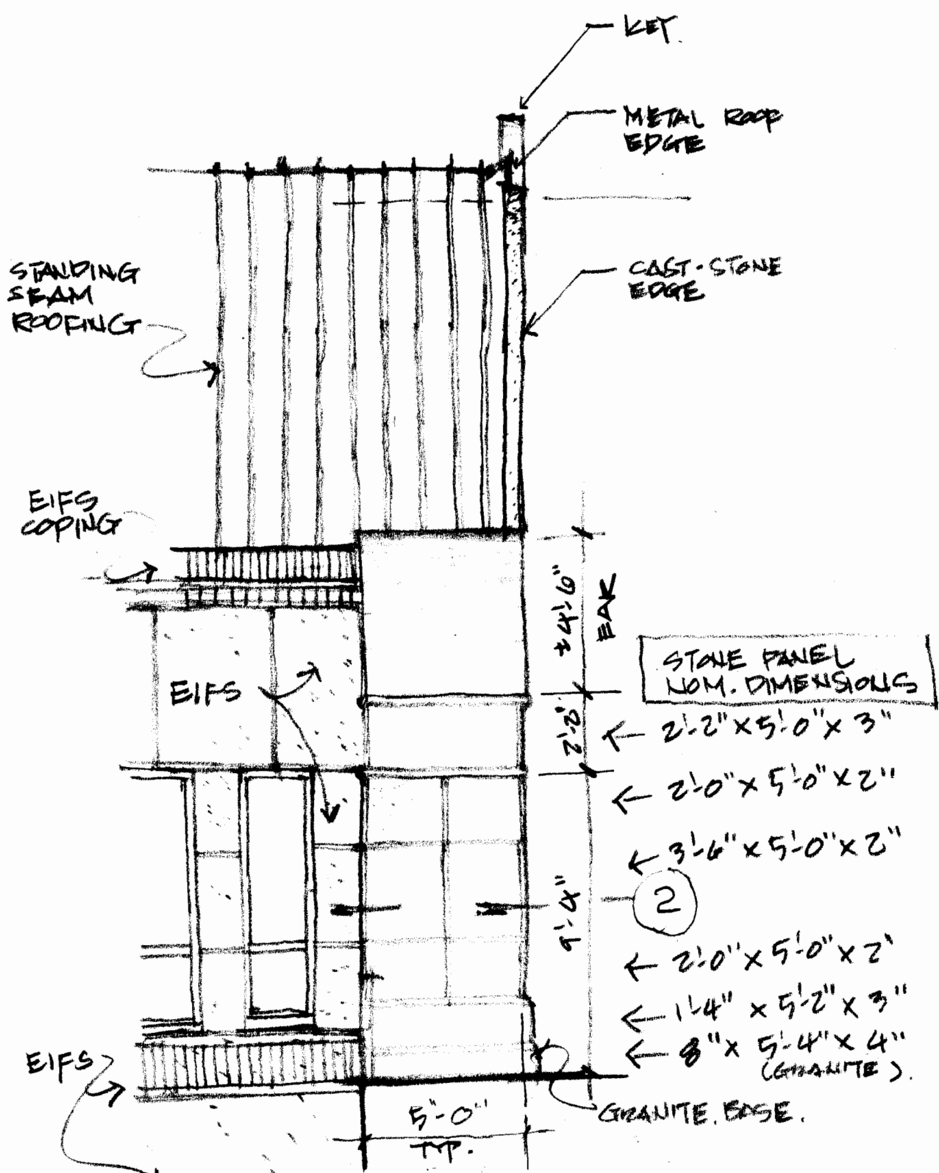
ELEVATION SOUTH 1/4"
