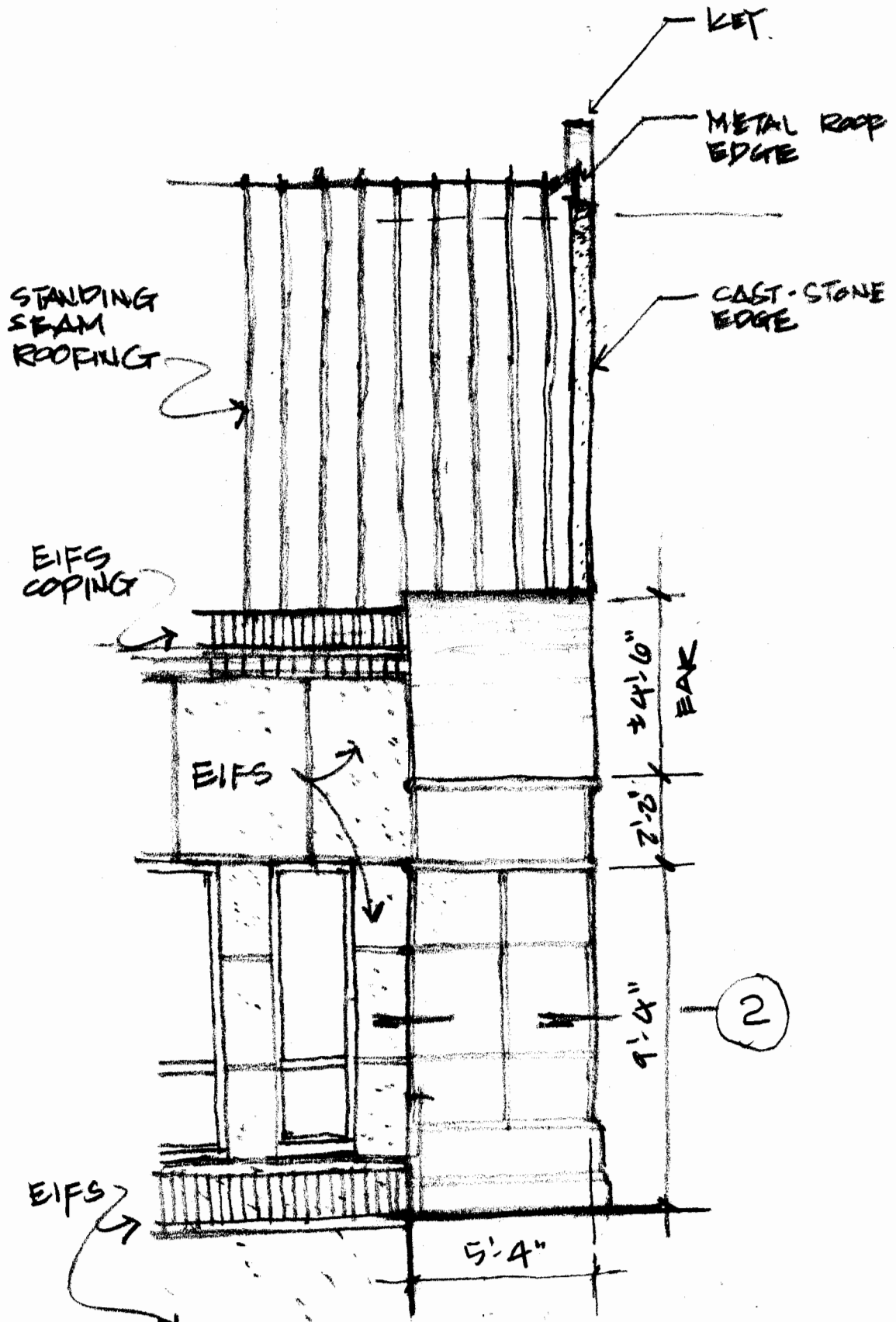
ELEVATION SOUTH 1/4"
